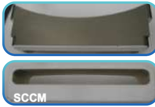
Liner Gate Hard D HP (Recoating) P/n 1810-225118-11
