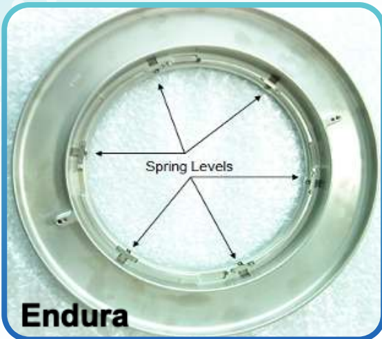
6 Pad Clamp Ring with Spring Lever P/n CT 433-01946-B
