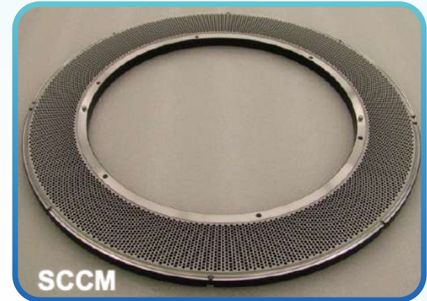
Plate, Exhaust P/n 3D10-100845-11
