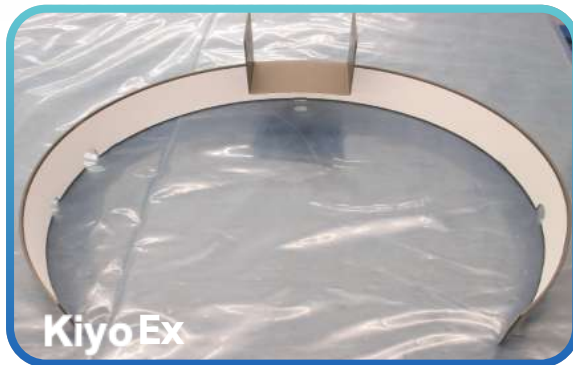
Liner Fixed OUTR ACME 2300 P/n 714-045743-809
