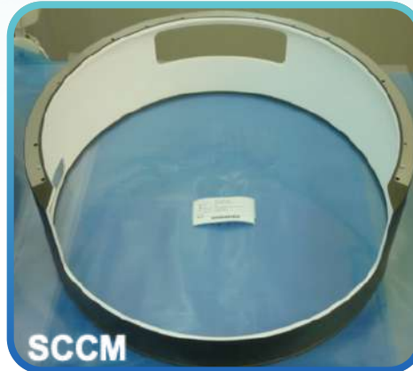
Recoating Shield Depo Up LLD-HP_ME Hi Power P/n 1D10-103187-11
