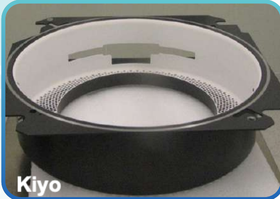
Kiyo Liner, Upper Chamber 2300 P/n 0806-4125-0030
