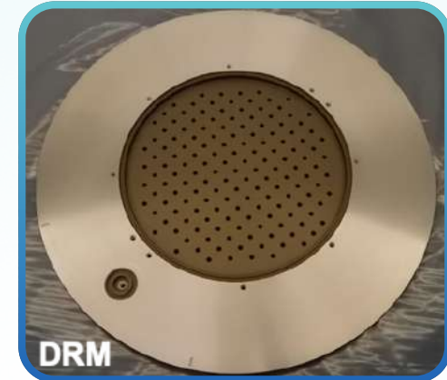
Upper Electrode P/n 3D10-100424-13
